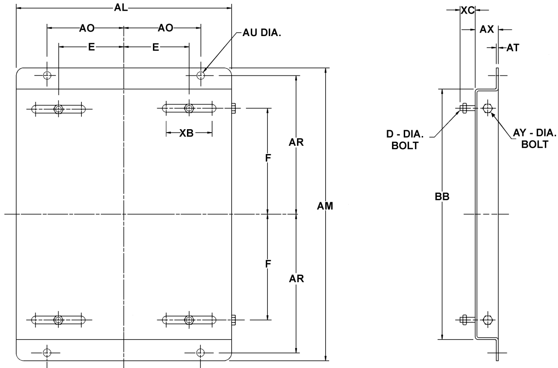
Adjustable Slide Base for Dynumatic Model AT-140 Through AT-440 Drives with Motor
